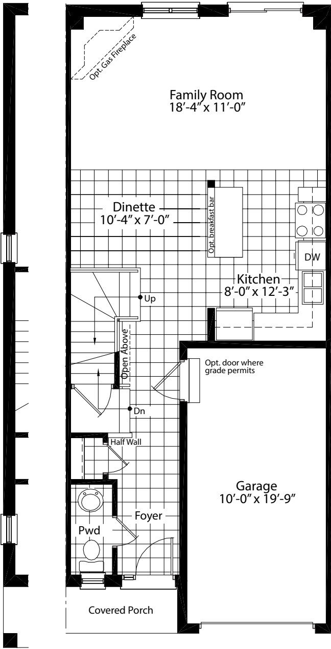
Main Floor Plan A 9'-0" main floor ceiling height
