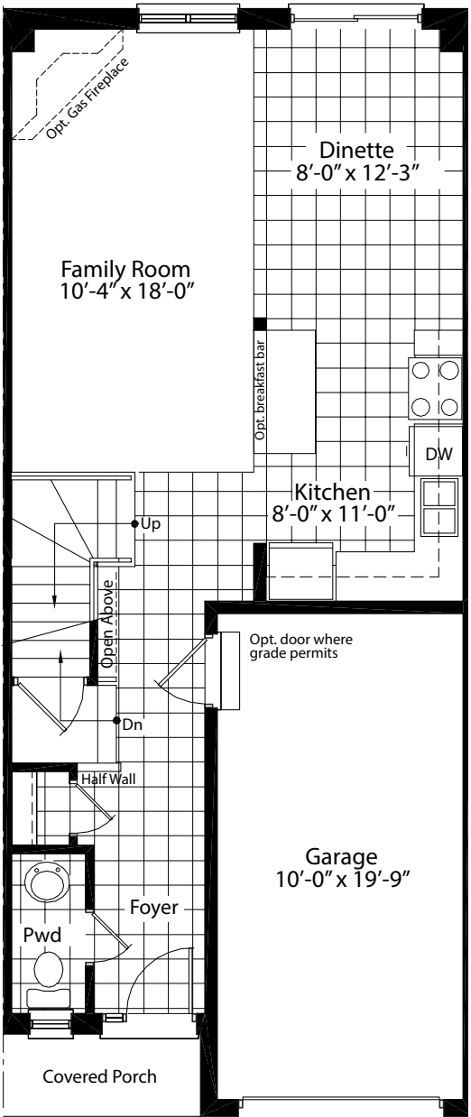
OPTIONAL Main Floor Plan B 9'-0" main floor ceiling height
