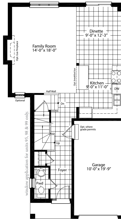
Main Floor Plan 9'-0" main floor ceiling height
