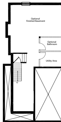
Basement Floor Plan
